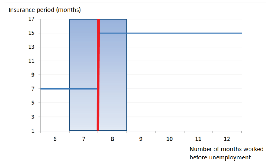
Figure 1 : Regression discontinuity
